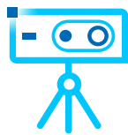
Multi-Camera AI
