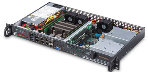
Intel® Select Solutions uCPE Base Configuration SYS-5019D-FN8TP
